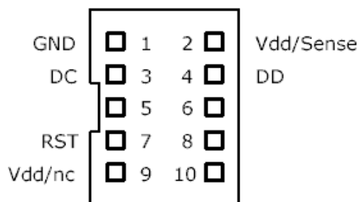
Header - Top View Figure 13.1
