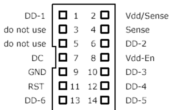
Header - Top View Figure 13.2
